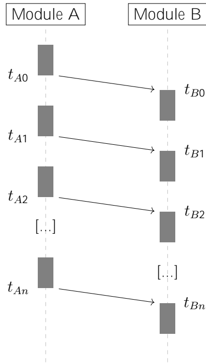
Figure 5.1: Sequence diagram of messages sent between two modules illustrating the setup used to determine the clock drift
